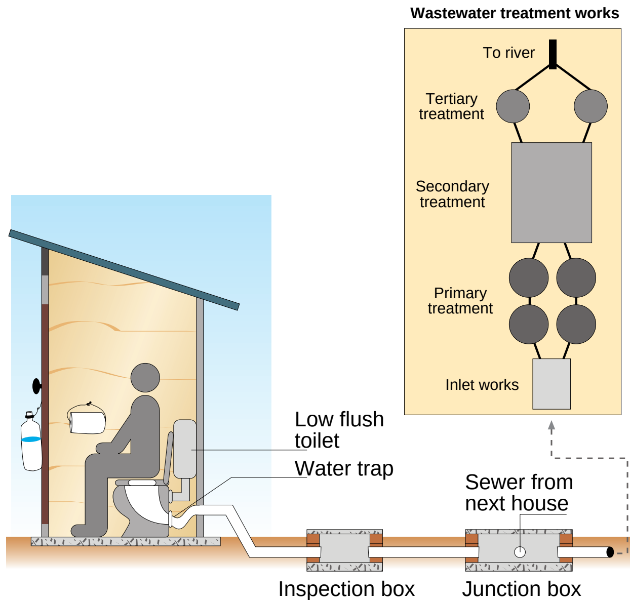
A toilet, usually in-house, flushed using lower volumes of water than either conventional sewerage or septic tanks, to smaller diameter sewers laid at flatter gradients and shallower depths between dwellings on a block. On-site shallow inspection chambers are provided.
