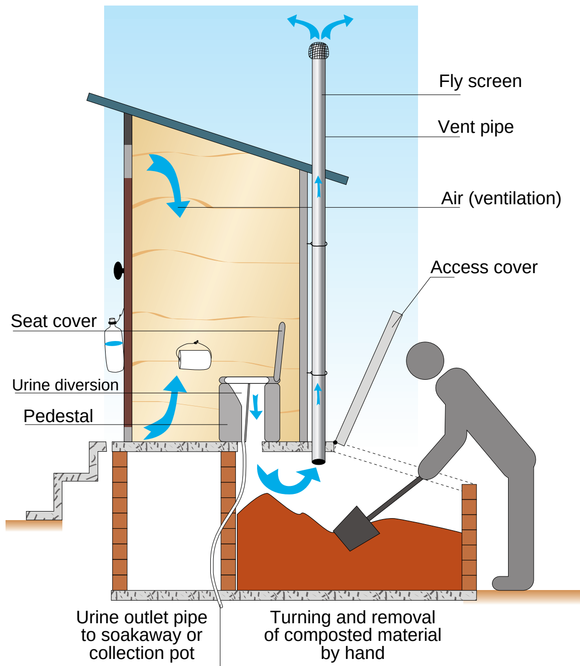
A single top-structure over a sealed container, which could be one of two chambers side by side (as for the VIDP), with access for the removal of decomposed waste. A vent pipe may be installed to encourage drying of the waste.
