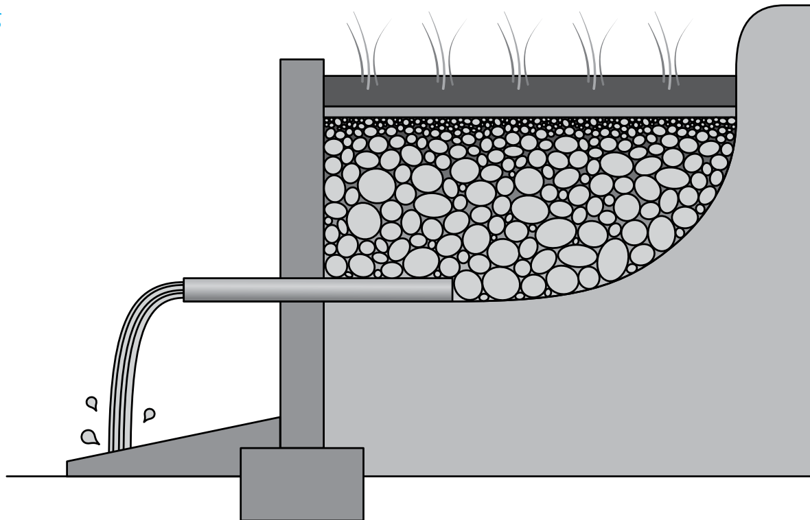
Fig 1: A protected spring
