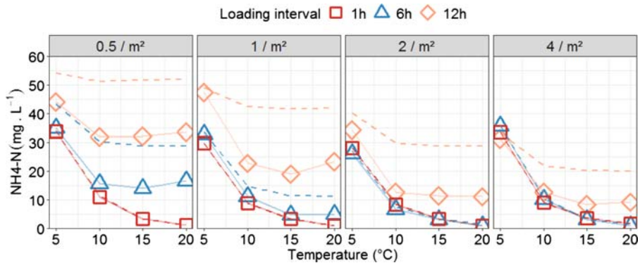
Figure 5.2 Simulated \text{NH}_4\text{-N} effluent concentrations of a VF filter with main layer of coarse sand (1–4 mm) for an OLR of 80 g COD/ \text{m}^2 /d for different loading intervals and different number of holes in the distribution pipes (median concentrations: symbols; maximum concentrations: dashed lines).
