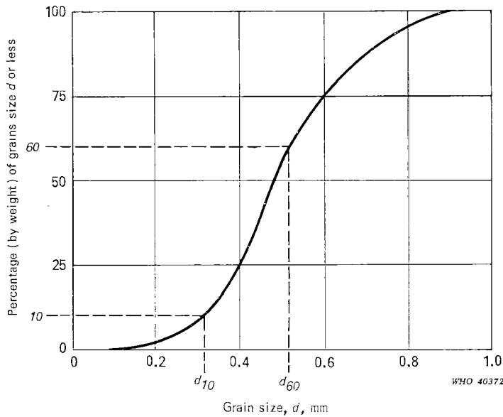
FIG. 5. SIEVE ANALYSIS
