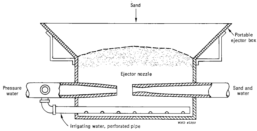
FIG. 32. HYDRAULIC SAND EJECTOR
