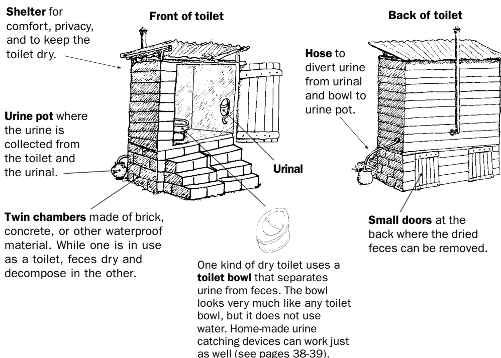
Parts of the twin chamber dry toilet
