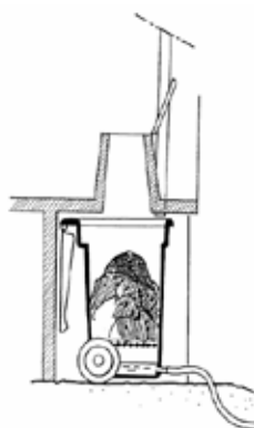
Figure 15. Schematic diagram of movable bin composting toilet (source: Winblad and Simpson-Hebert (2004)).
