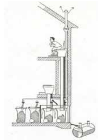
Figure 19. Sketch of the movable bin system at Gebers apartment block in Stockholm, Sweden (source: Winblad and Simpson-Hebert (2004).
