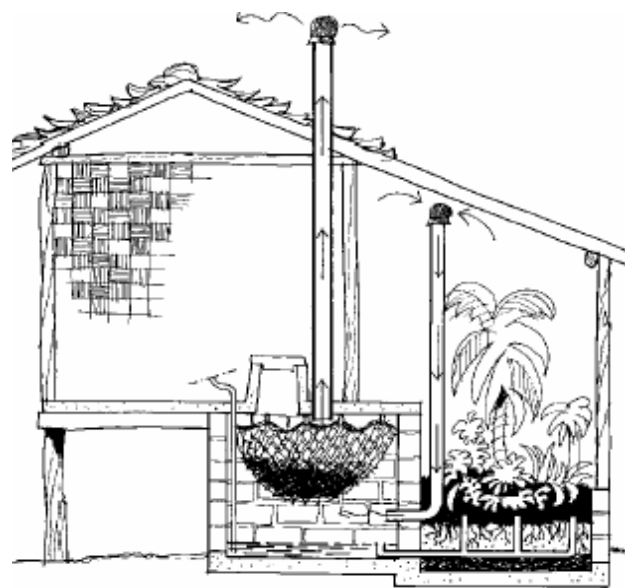
Figure 12. Cross section of the CCD composting toilet with attached greenhouse and evapo-transpiration bed (source: Winblad and Simpson-Hebert (2004)).
