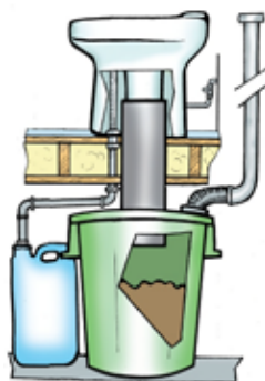
Figure 13. Urine diverting dry toilet with bucket under floor (source: Wostman Ecology AB, Sweden)
