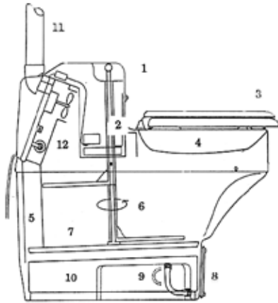
Figure 22. Cross section of a compact toilet with vertical stirring unit (source: Biolet USA/Switzerland)
