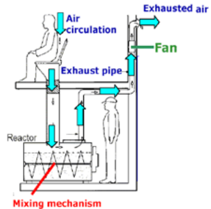
Figure 21. Cross section of a toilet facility with horizontal stirring unit (source: Seiwa Denko, Japan)
