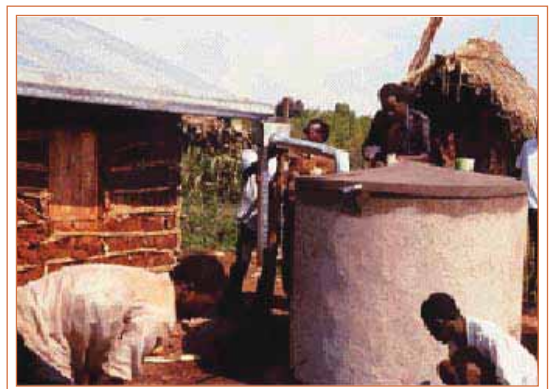
Rainwater tanks constructed by local builders called 'fundis' in Kenya
