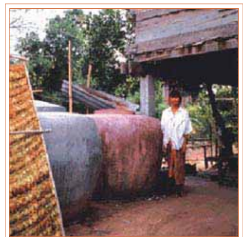
Thai Jar: RWH System in Thailand
