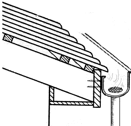
Figure 25: Coarse filter
