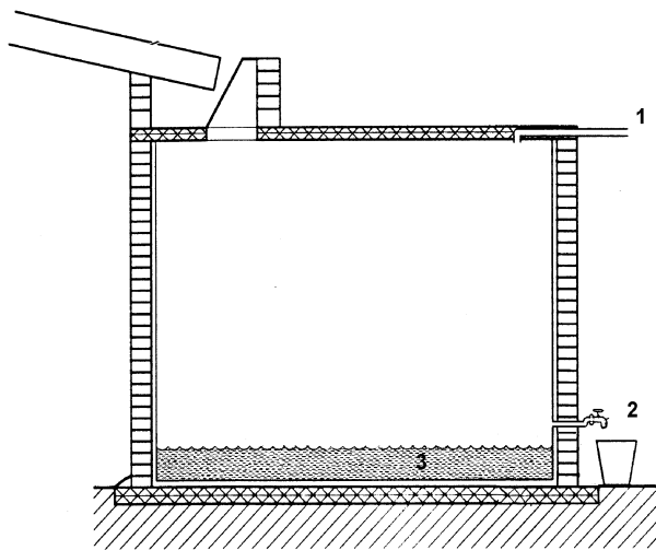
Figure 17: Overflow (1), Tap device (2), Dead storage (3)
