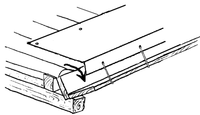
Figure 13: Splash guards
