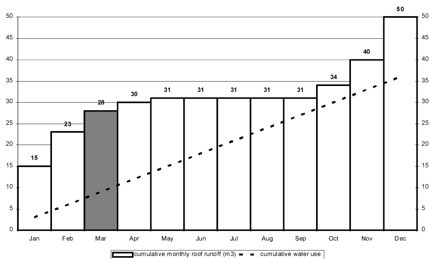
Figure 16: Cumulative monthly roof run-off including a residual storage of 5 m 3 and cumulative water use. Estimation of storage requirement.
