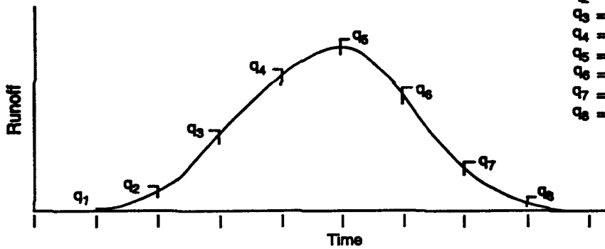
Runoff Hydrograph
