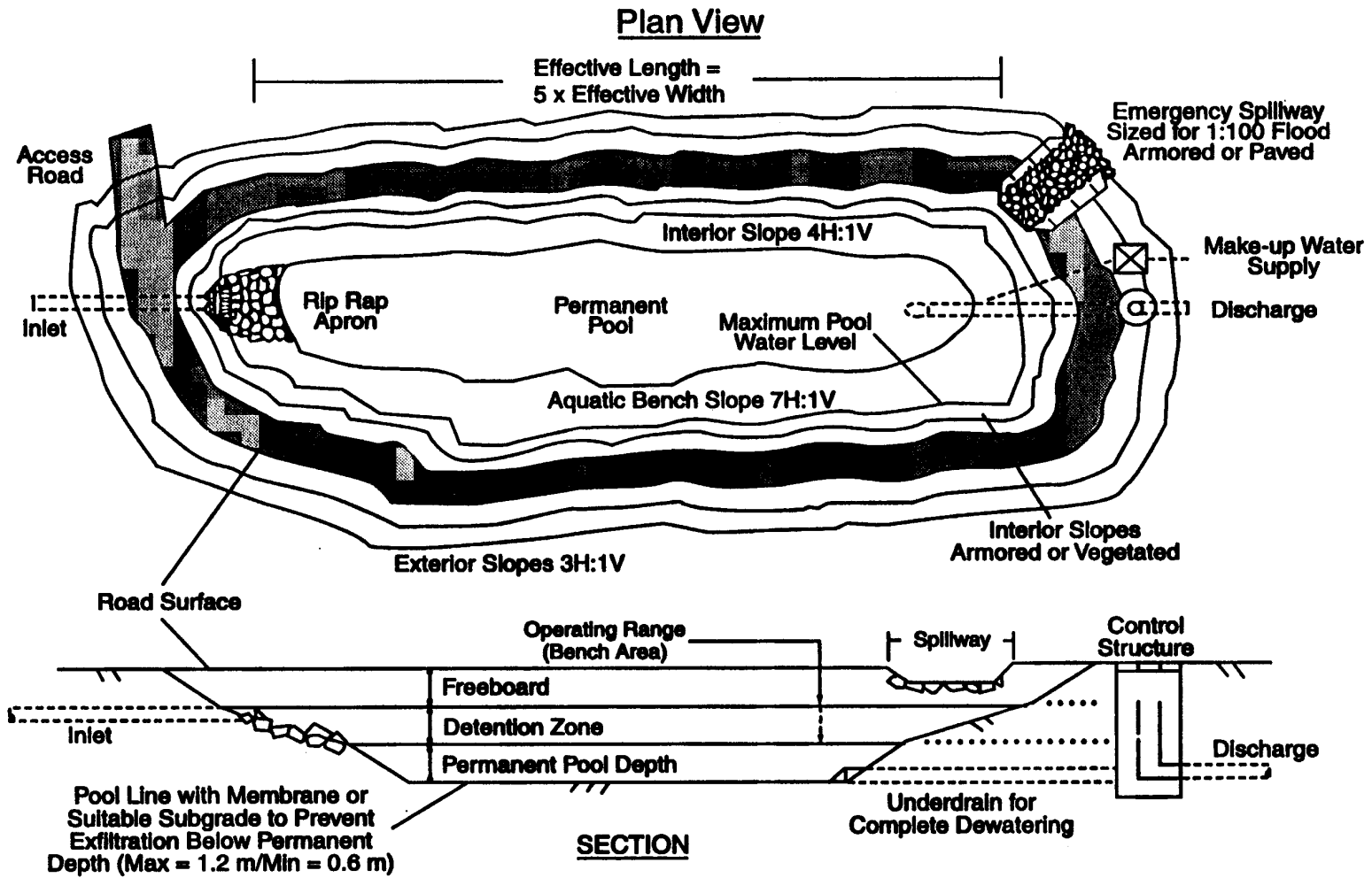
Figure 6.10 Wet Detention Pond Plan and Sections
