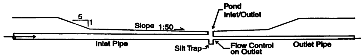
DRY STORMWATER DETENTION POND
