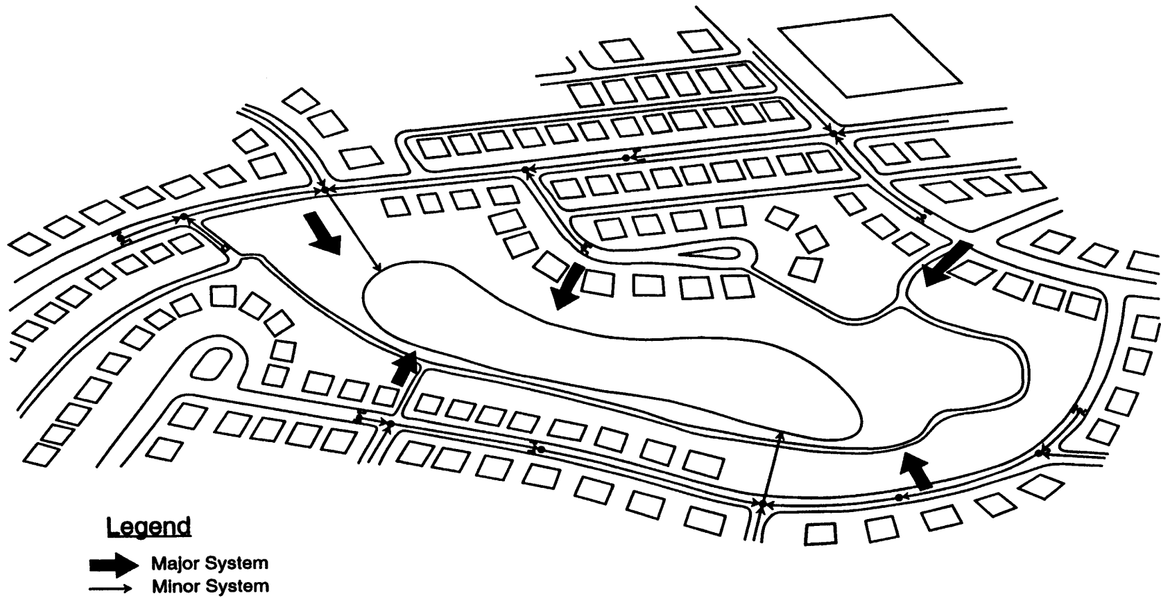
Figure 3.1 Major/Minor Systems
