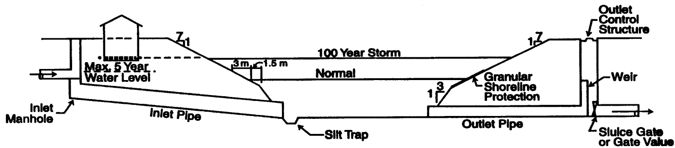
WET STORMWATER DETENTION POND
