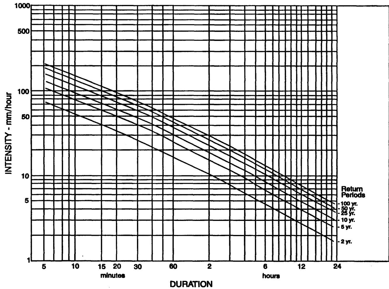
Figure 4.1 Typical I.D.F. Curve Format
