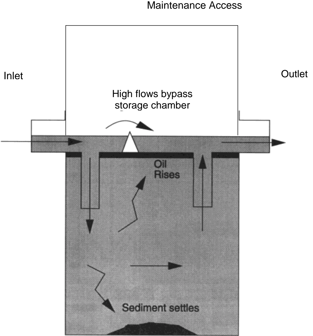
Figure 6-19 Bypass Separator
