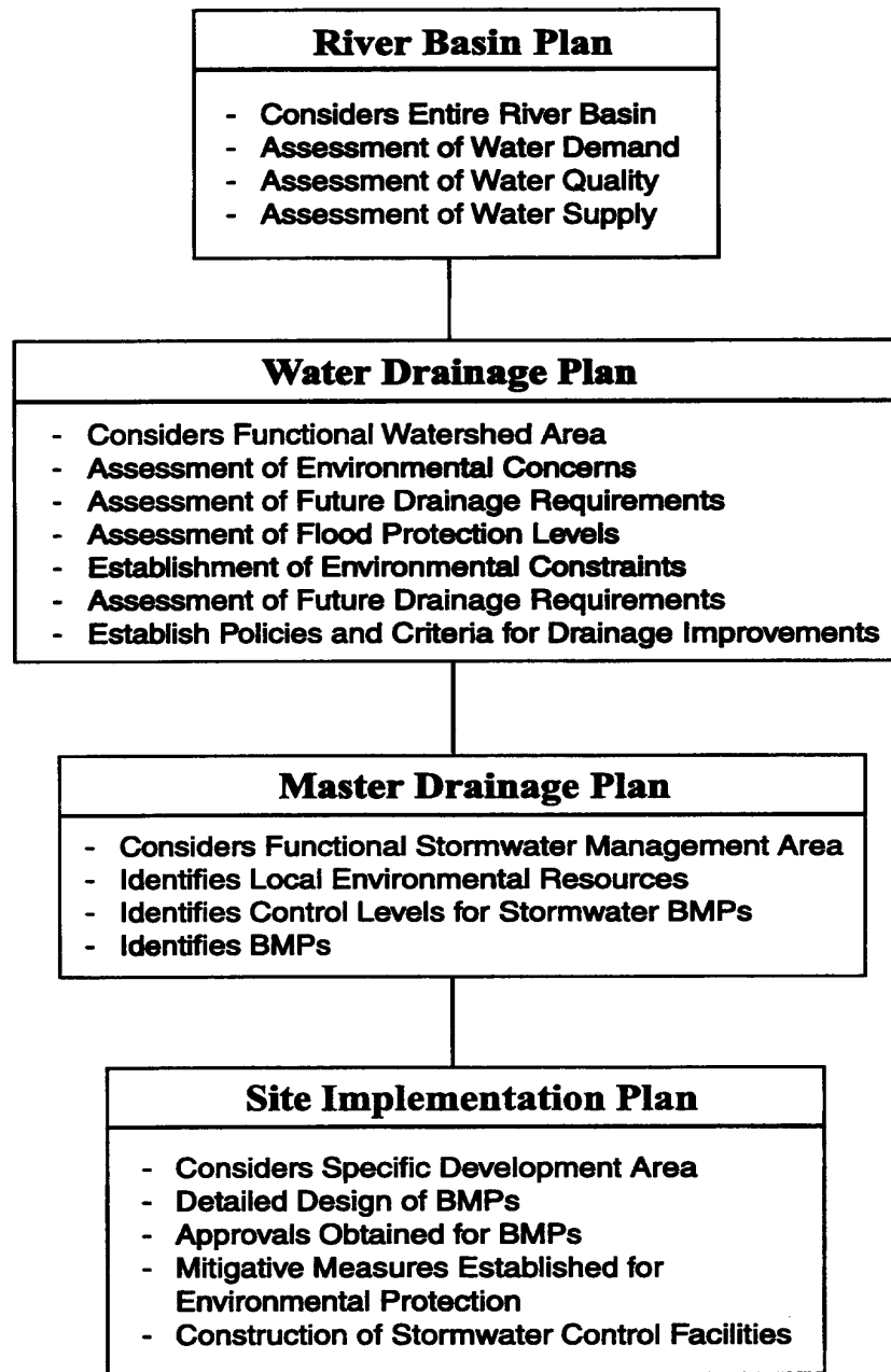
Figure 2.2 Functional Relationship of the Four Levels of Stormwater Management
